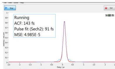
AUTOCORRELATION TRACE
